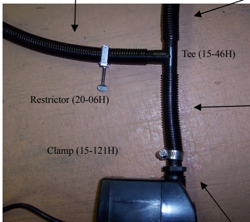
Pump (24-68H)
